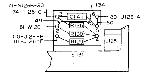
VIEW AT "B-B" ROTATED 180°
